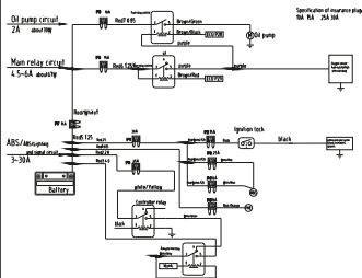
Sa 180 14-way insurance and control relay diagram
